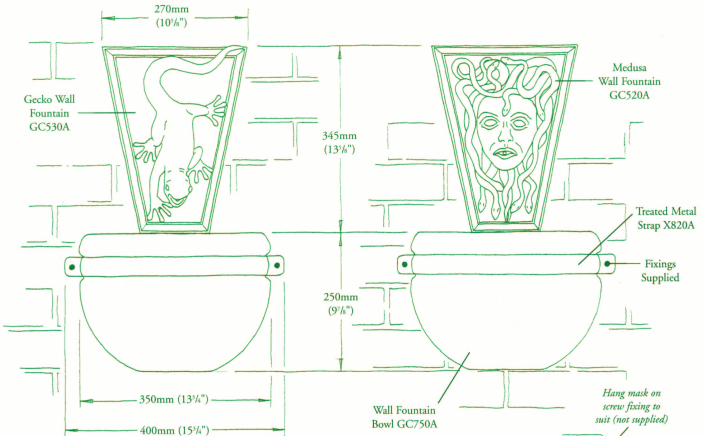
ELEVATIONS
