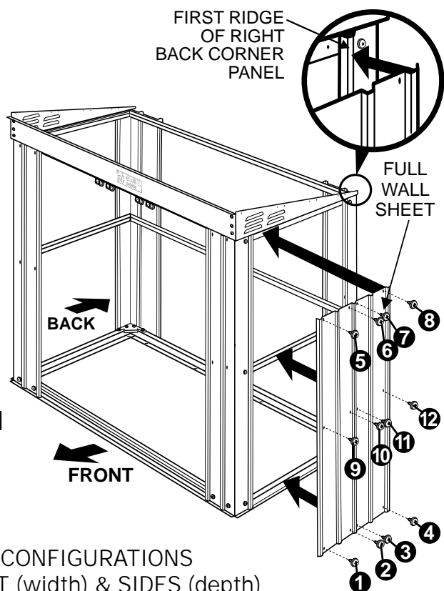
Diagram 13A 3' Deep Shed
