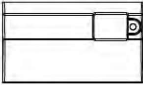
CVS (x1)
