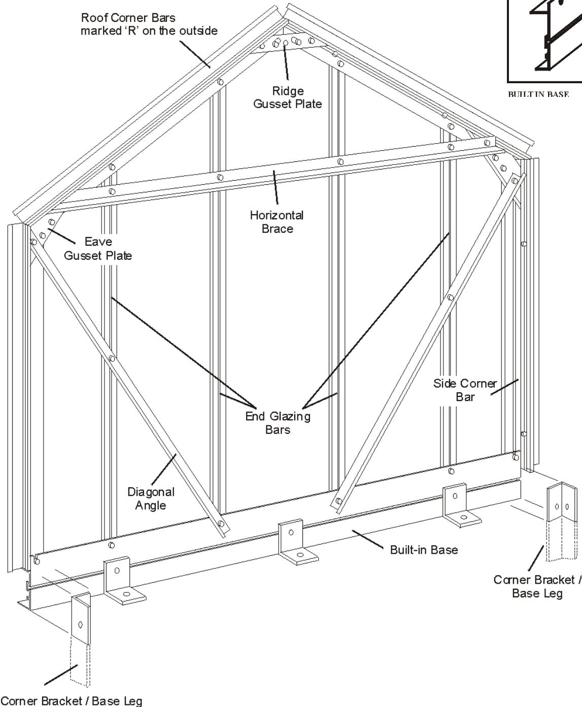
BRACING ANGLE
