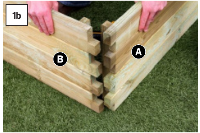
Interlock End Panels A with Side Panels B (Figs.1a & 1b) to form a rectangular planter.
