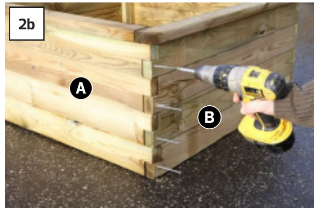
Secure in position using 8no Screws - 2no per internal corner (Fig.2a) and 12no screws - 3no per external corner (Fig.2b).
